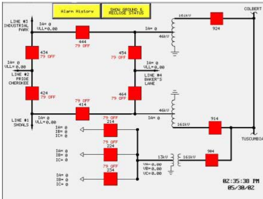
Figure 2: Example System Single Line
