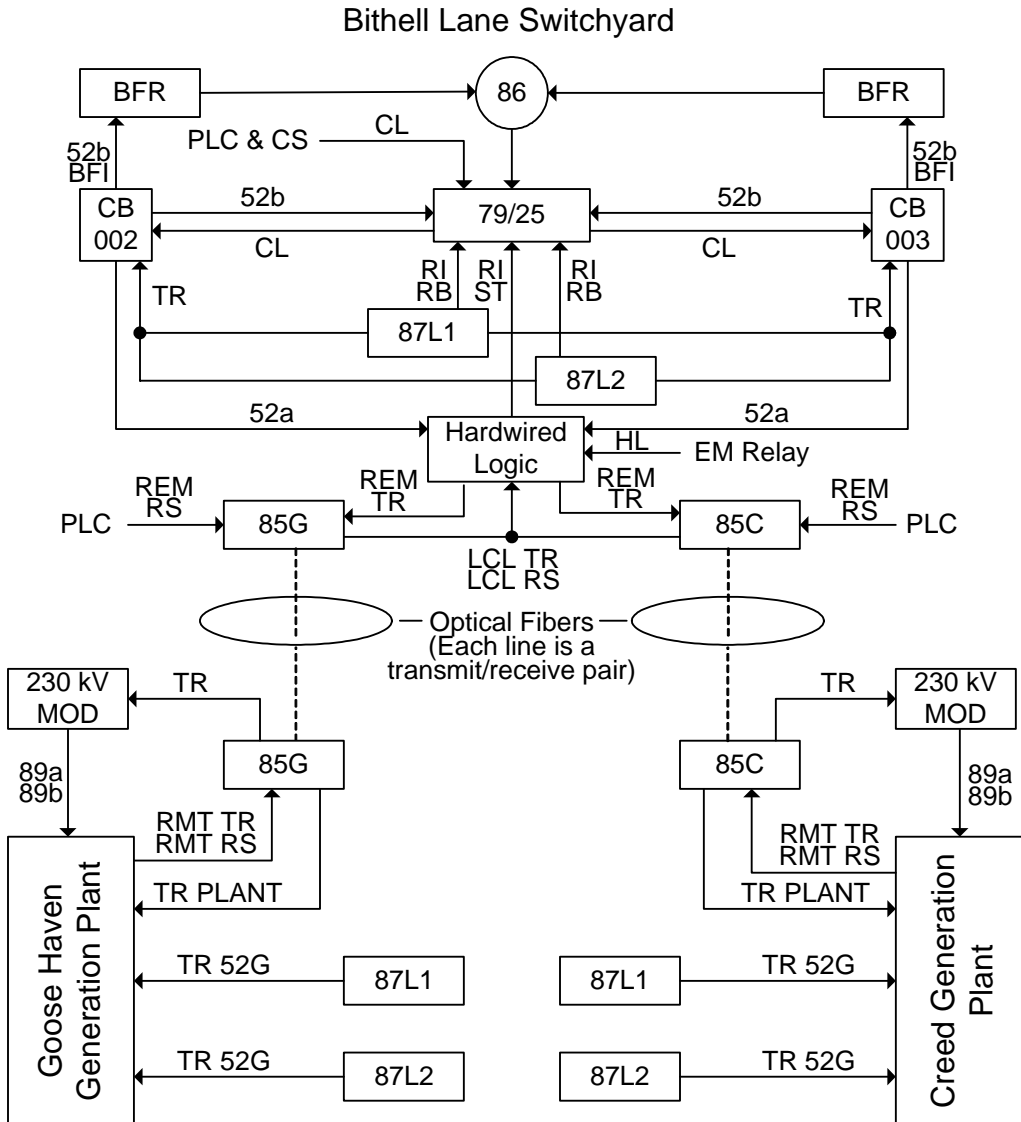
Figure 3. Protection and Restoration System Block Diagram
