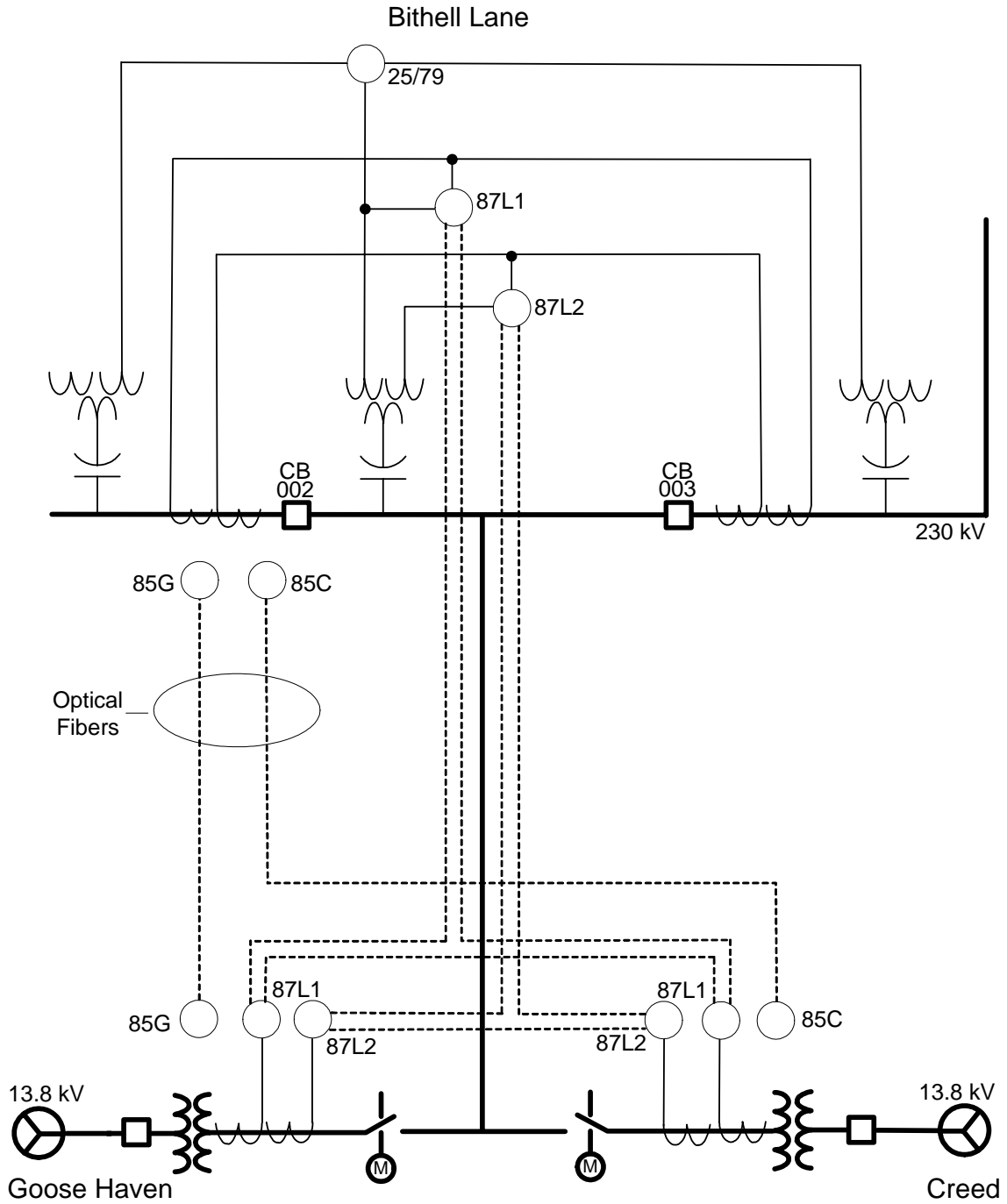
Figure 2. Protection and Restoration System Single Line Diagram
